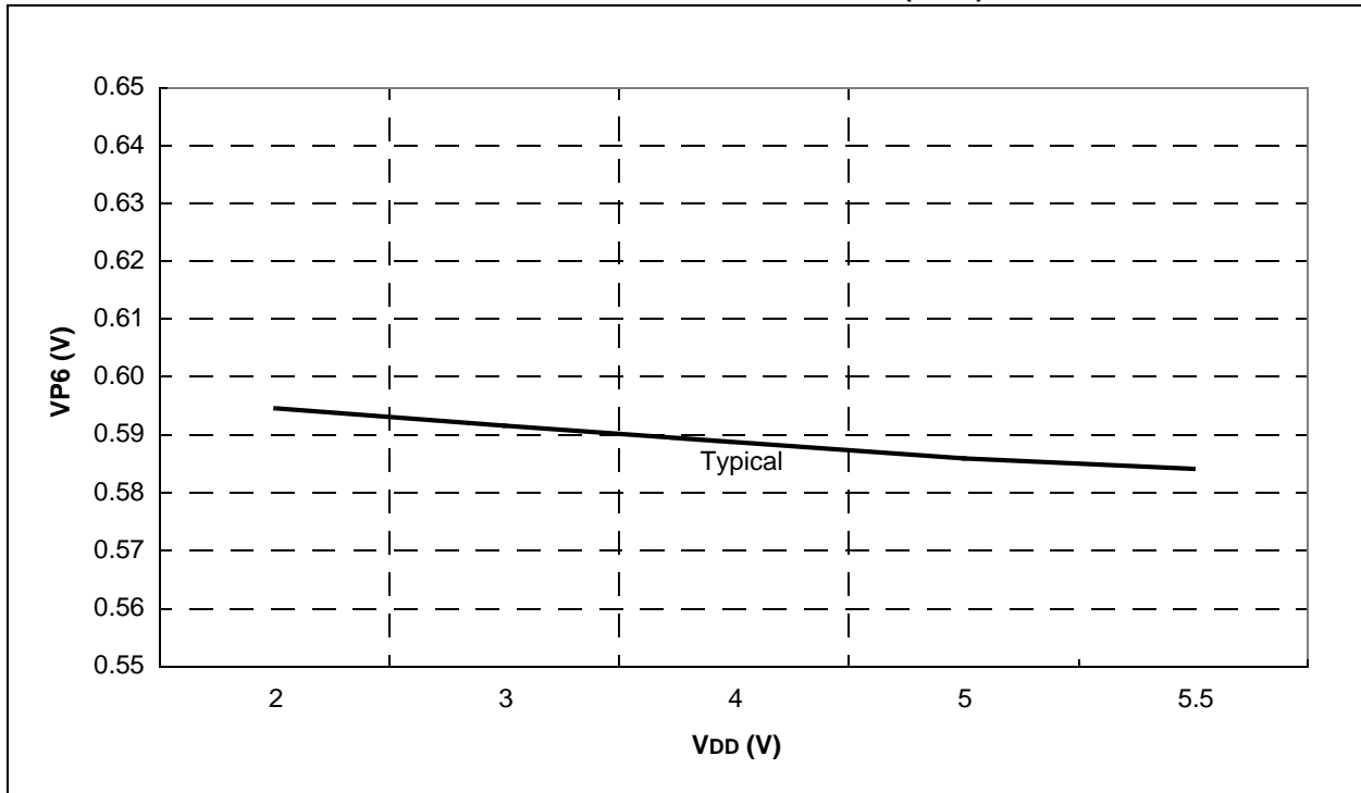
FIGURE 18-43: TYPICAL VP6 REFERENCE VOLTAGE vs. V_{DD} ( 25^{\circ}\text{C} )
