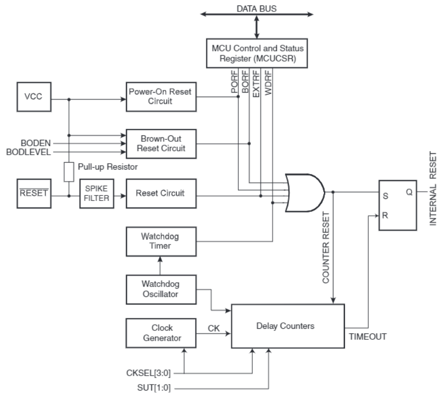
Figure 10-1. Reset Logic
