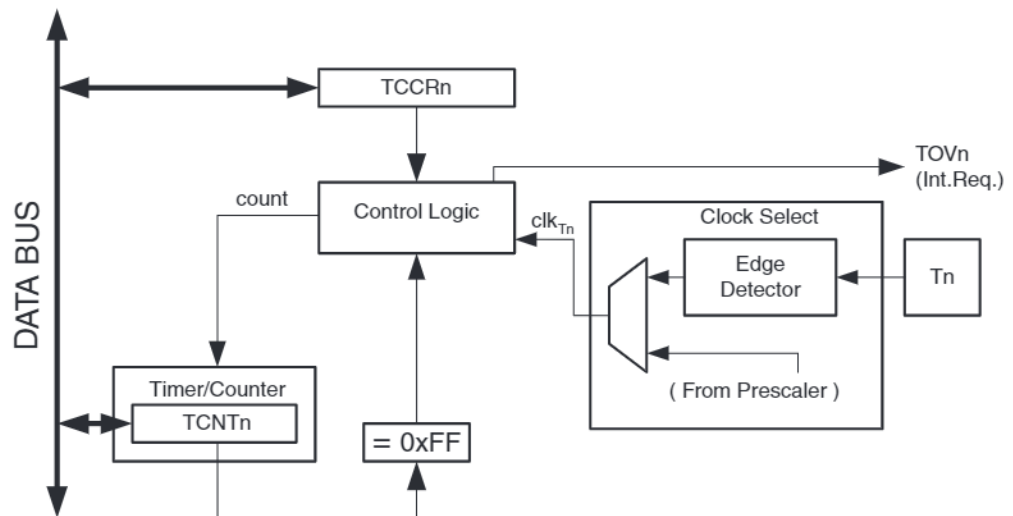
Figure 14-1. 8-bit Timer/Counter Block Diagram
