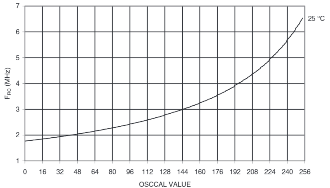
Figure 26-57. Calibrated 4 MHz RC Oscillator Frequency vs. Oscscal Value
