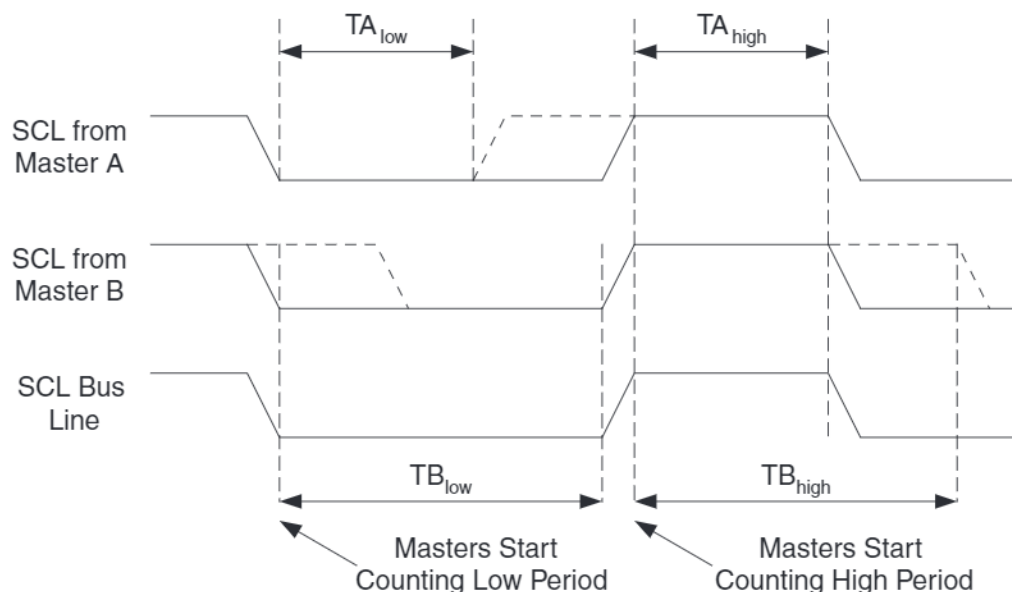
Figure 20-8. SCL Synchronization Between Multiple Masters
