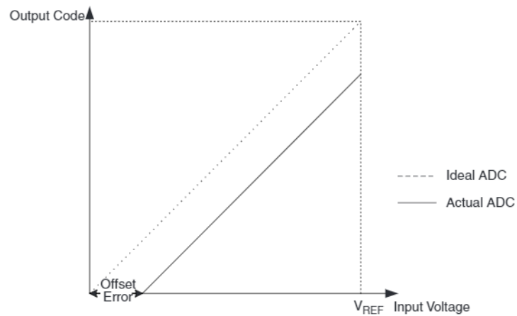
Figure 22-8. Offset Error
