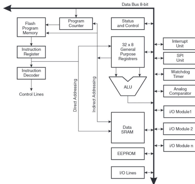
Figure 6-1. Block Diagram of the AVR MCU Architecture
