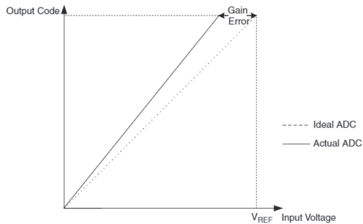
Figure 22-9. Gain Error
