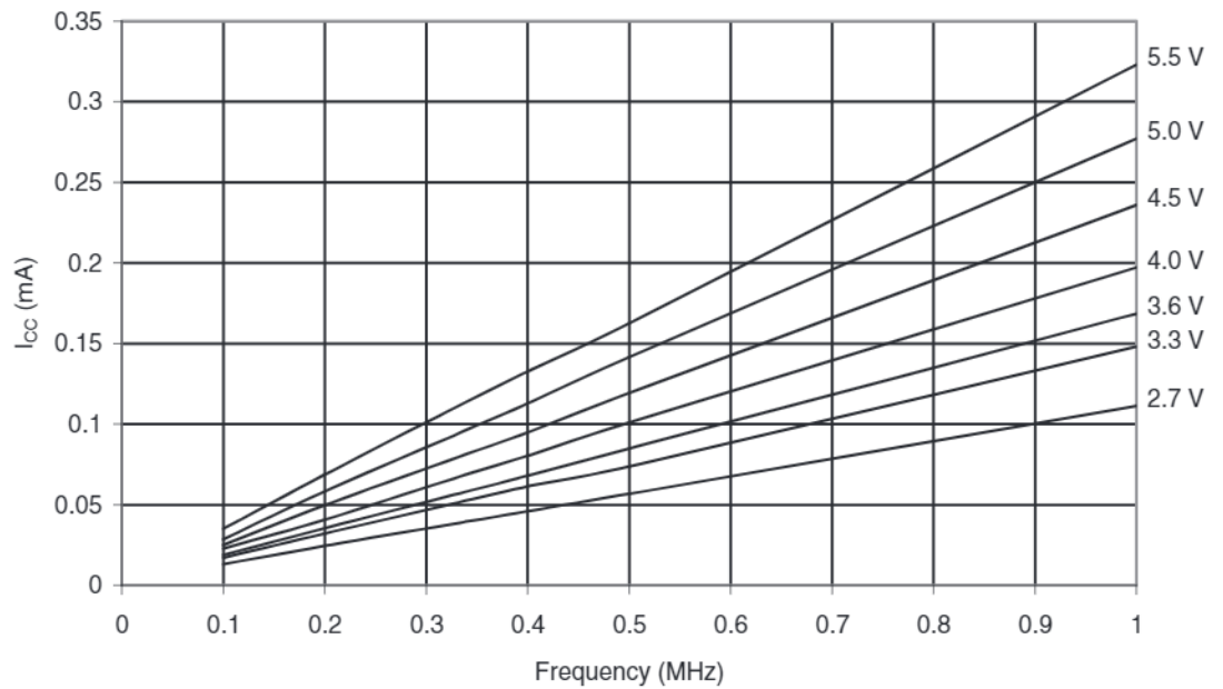
Figure 26-8. Idle Supply Current vs. Frequency (0.1 - 1.0 MHz)
