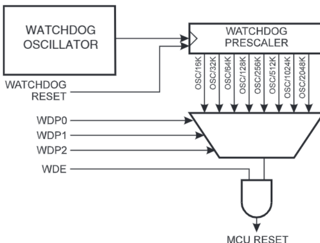
Figure 10-7. Watchdog Timer
