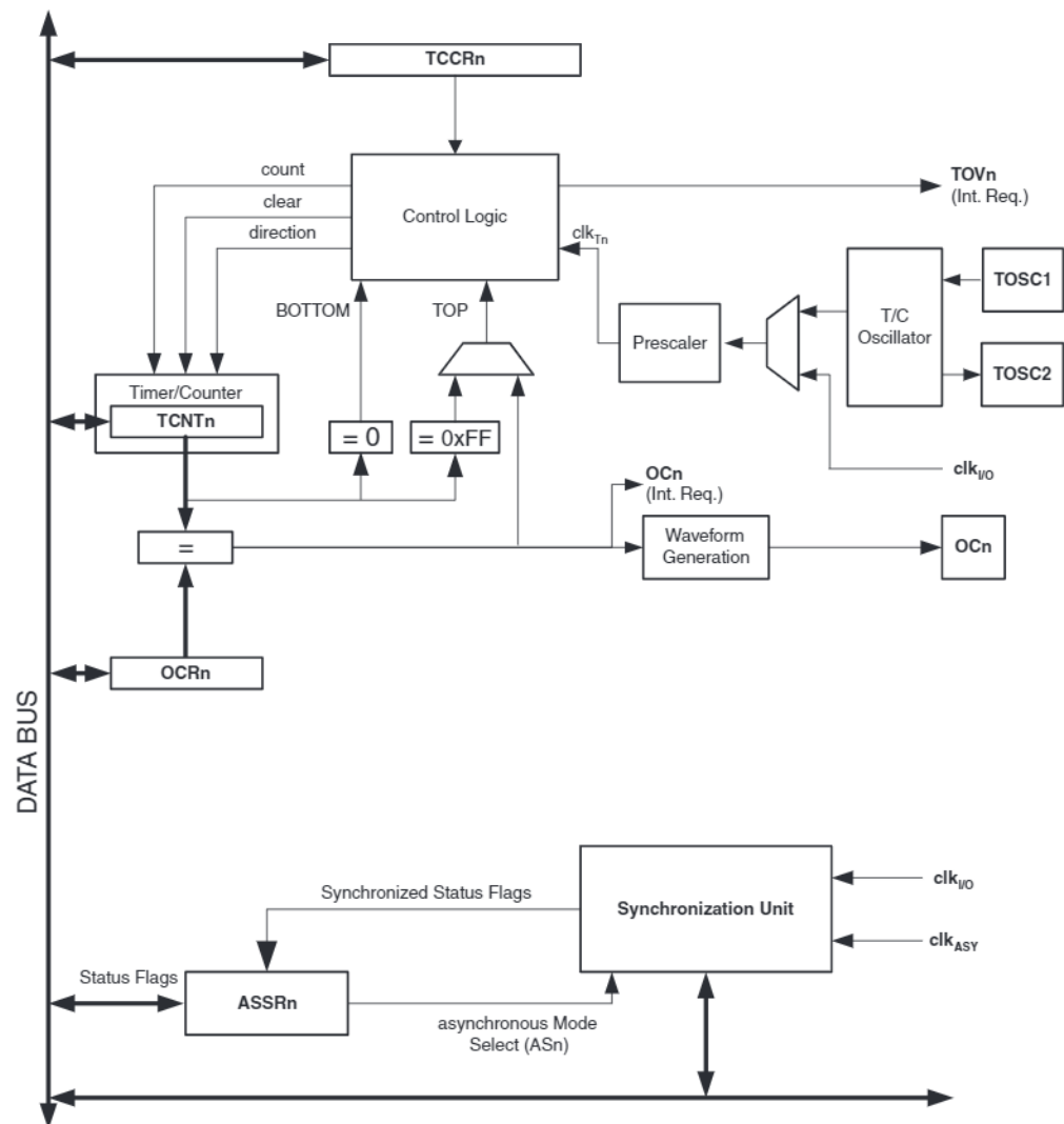
Figure 17-1. 8-bit Timer/Counter Block Diagram
