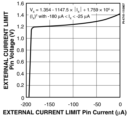
Figure 45. EXTERNAL CURRENT LIMIT Pin Voltage vs. Current.
