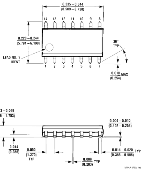
Molded Small-Outline Package (M) Order Number LF298M or LF398M NS Package Number M14A
