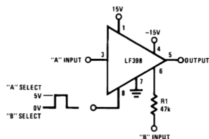
2-Channel Switch
