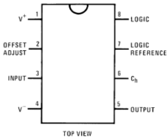
Dual-In-Line Package
