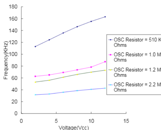
Decoder (PT2270) OSC Frequency
