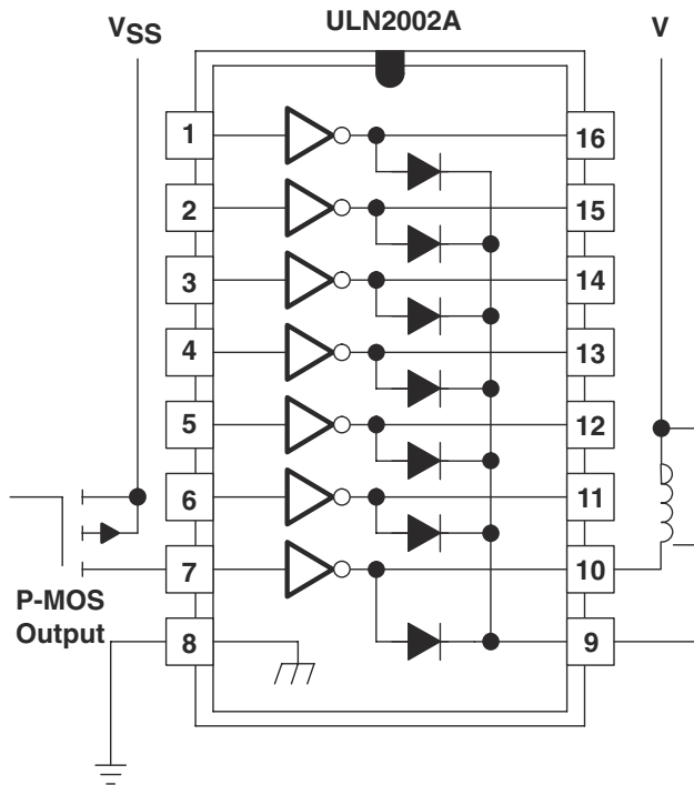
Figure 9-4. P-MOS to Load
