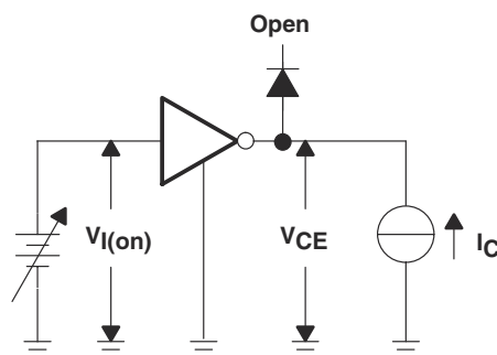
Figure 7-6. V_{I(on)} Test Circuit
