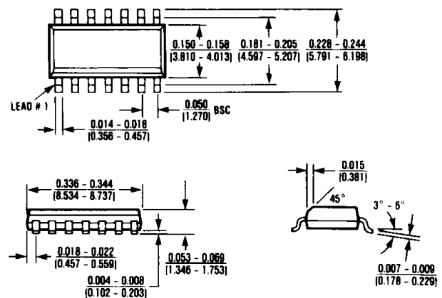
14 Lead Small Outline (SD)
