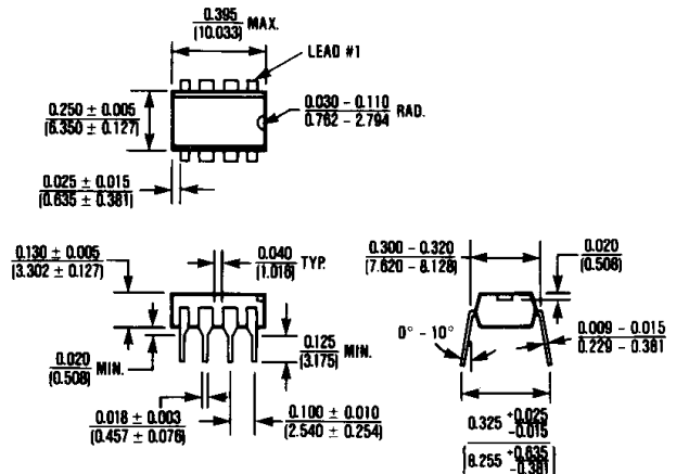
8 Lead Plastic DIP (PA)
