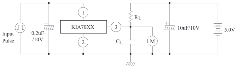
APPLICATION CIRCUIT
