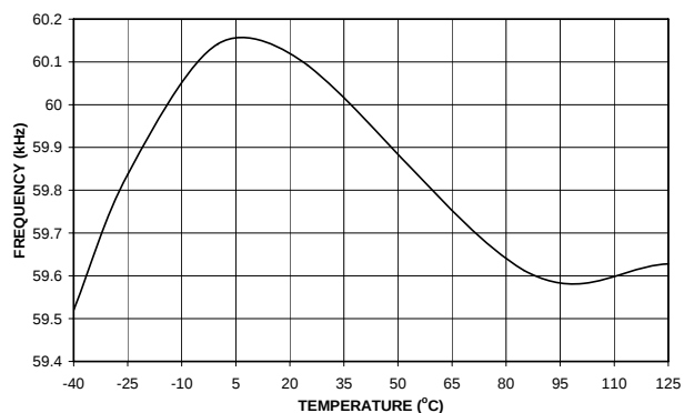
Figure 5. Fsw min
