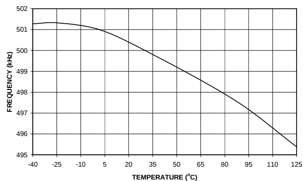
Figure 20. Fsw max
