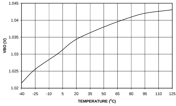
Figure 15. Brown-Out Reference (VBO)
