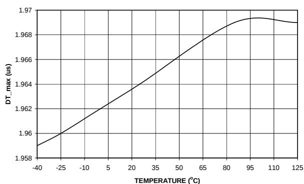
Figure 13. T_dead_max
