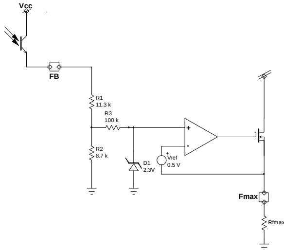
Figure 32. The OPAMP Arrangement limits the VCO modulation signal between 0.5 and 2.3V
