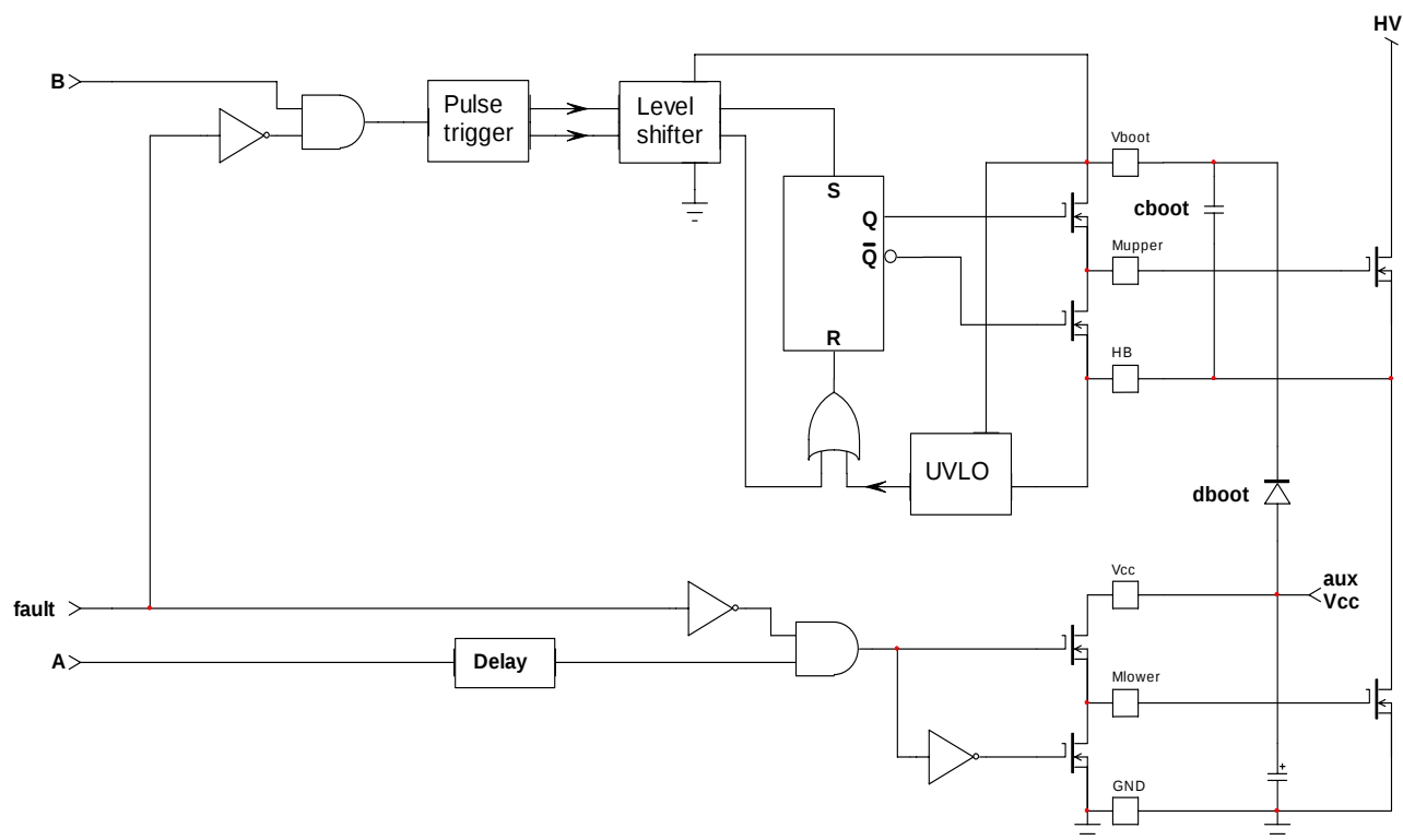
Figure 51. The Internal High-voltage Section of the NCP1396
