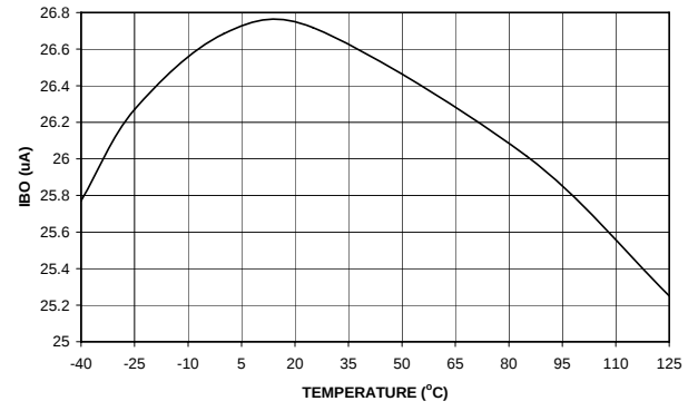
Figure 16. Brown-Out Hysteresis Current (IBO)
