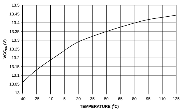
Figure 3. VCC ON
