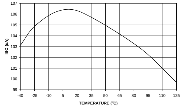
Figure 30. Brown-Out Hysteresis Current (IBO)
