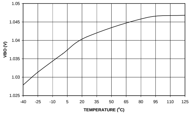
Figure 29. Brown-Out Reference (VBO)
