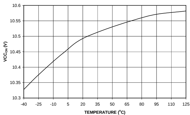
Figure 17. VCC ON
