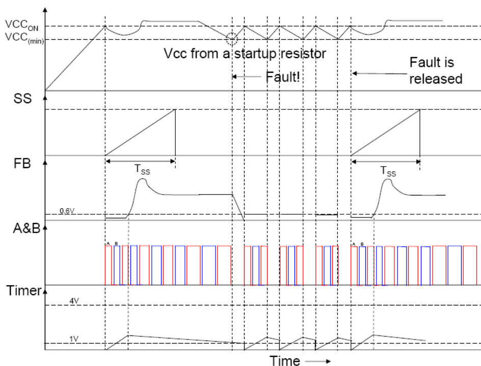
Figure 50. When the V_{CC} is too low, all pulses are stopped until V_{CC} goes back to the startup voltage
