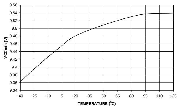
Figure 4. VCC(min)
