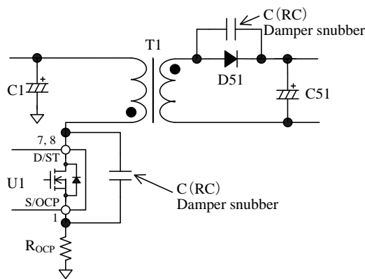
Figure 9-18 Damper snubber
