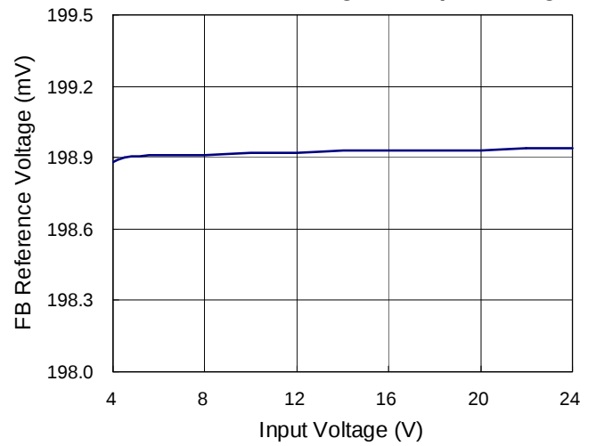
FB Reference Voltage vs. Input Voltage
