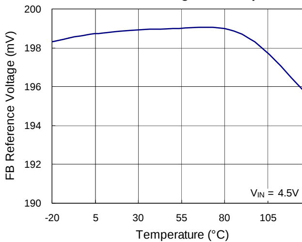
FB Reference Voltage vs. Temperature
