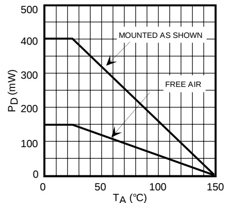
SOT23-3 POWER DISSIPATION CURVE
