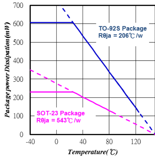
Figure 8. Power Dissipation vs. Temperature
