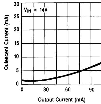
Quiescent Current
