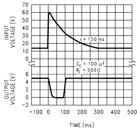
Operation During Load Dump
