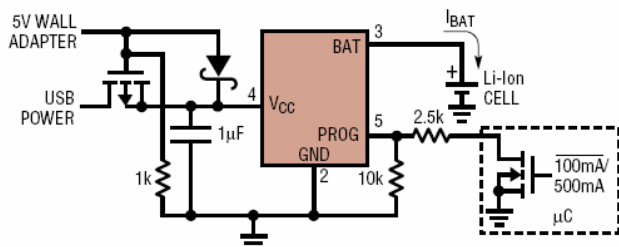
USB/Wall Adapter Power Li-Ion Charger
