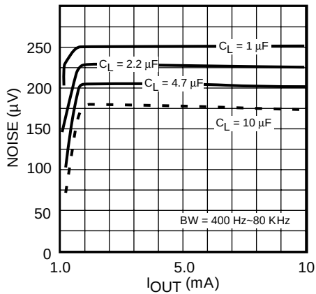
NOISE LEVEL (TK71530A) vs. OUTPUT CURRENT
