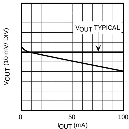
LOAD REGULATION
