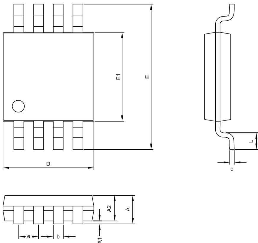
MSOP-8 Package
