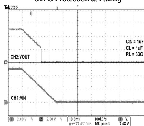
UVLO Protection at Falling
