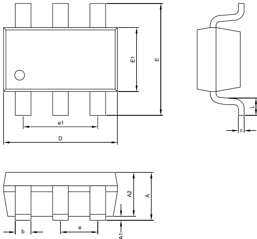
SOT-23-6 Package
