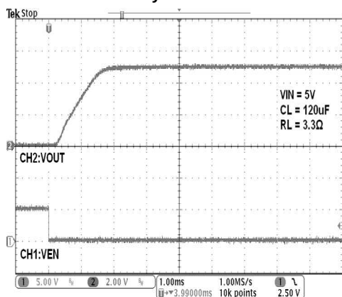
Turn on Delay Time and Rise Time
