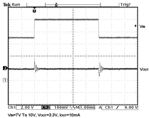
Line Transient
