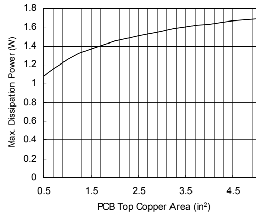
SOT-89 Max. Power Dissipation vs. PCB Top Copper Area
