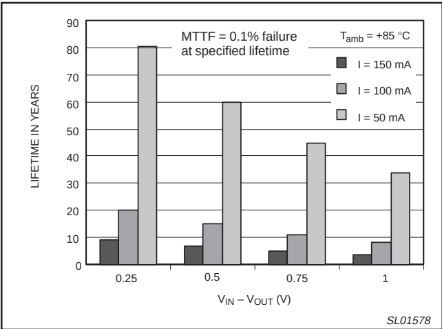
Figure 12. Lifetime versus V_{IN} - V_{OUT} for 3 output currents.
