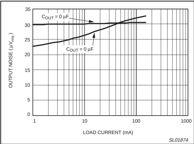
Figure 10. Output noise versus load current.
