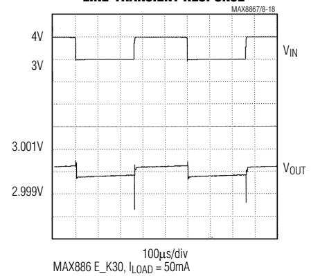
LINE-TRANSIENT RESPONSE
