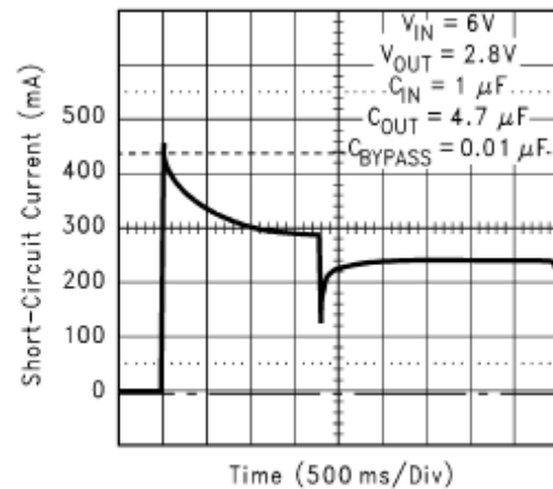
Short-Circuit Current
