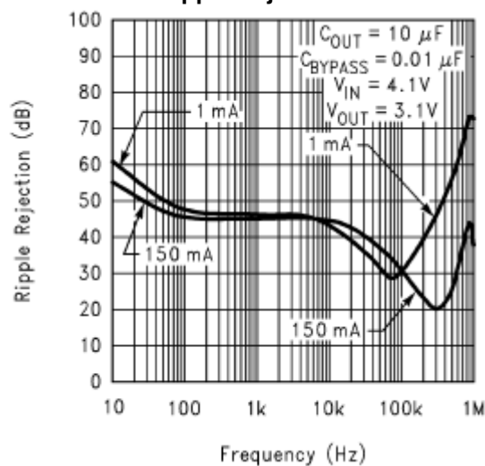
Ripple Rejection
