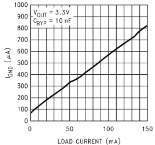
Ground Pin vs Load Current
