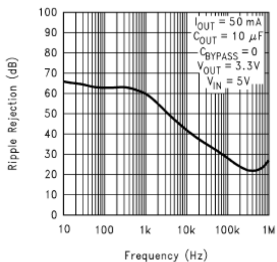
Ripple Rejection
