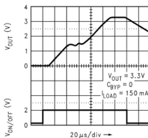
Turn-On Time
