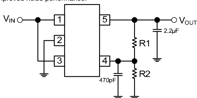
Application Circuit
