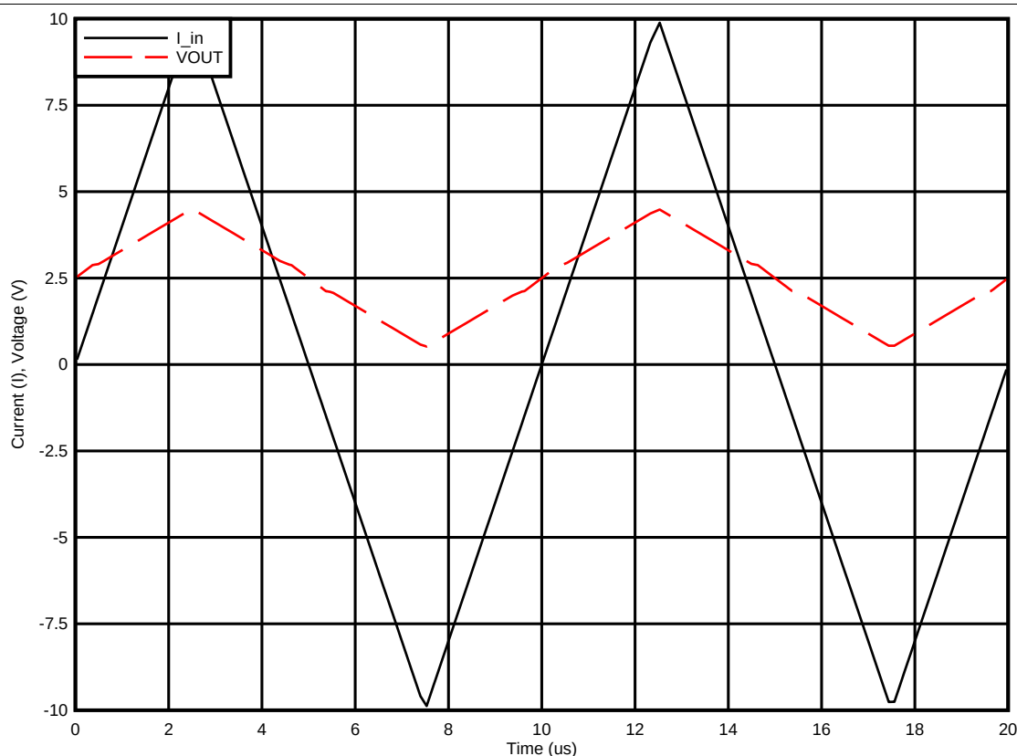
Figure 30. Output Voltage vs Shunt Input Current
