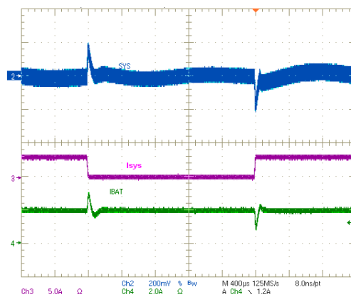
CH2: system voltage (AC), 200mV/div; CH3: system load current, 5A/div; CH4: battery charge current, 2A/div, 400μs/div Figure 12. 0-3A System Load Transient (IDPM Enable and Charge Enable)
