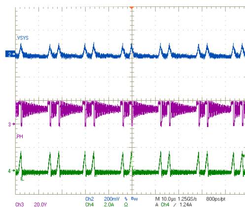
CH2: system voltage (AC), 200mV/div; CH3: PHASE, 20V/div; CH4: inductor current, 2A/div, 10μs/div
