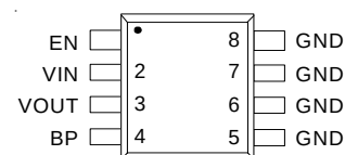
SOP-8
