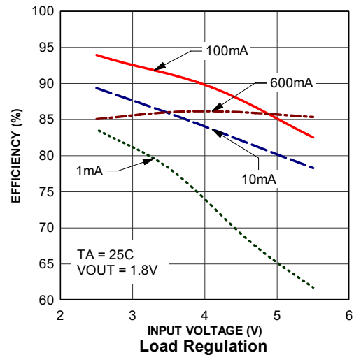
Efficiency vs Input Voltage
