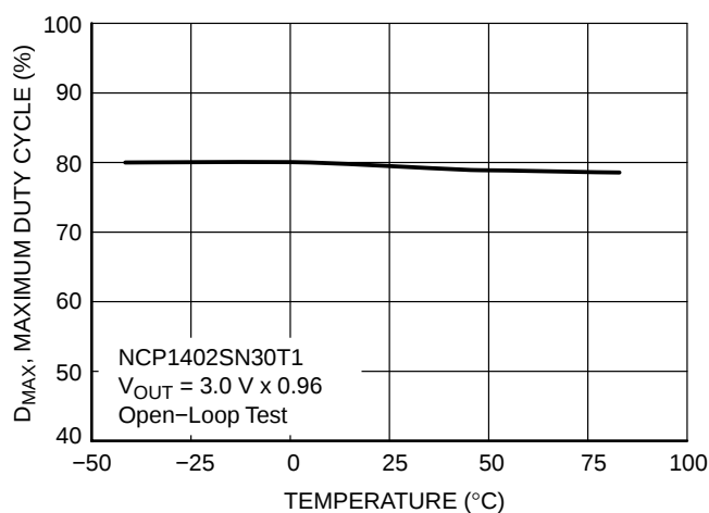
Figure 22. NCP1402SN30T1 Maximum Duty Cycle vs. Temperature
