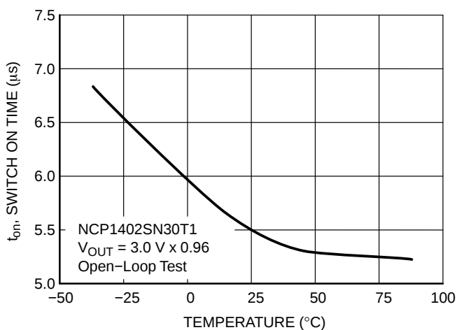
Figure 16. NCP1402SN30T1 Switch On Time vs. Temperature
