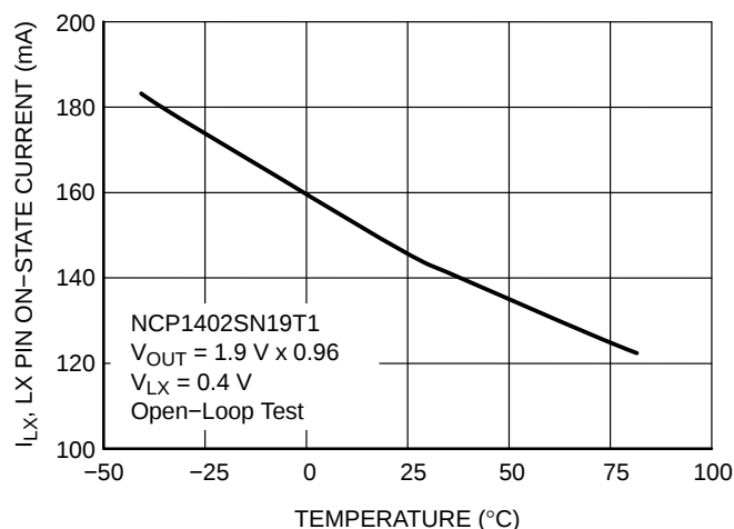
Figure 24. NCP1402SN19T1 LX Pin On-State Current vs. Temperature
