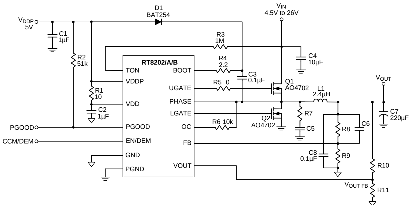
Figure 2. Output Voltage Setting for V_{OUT} > 3.3V Application
