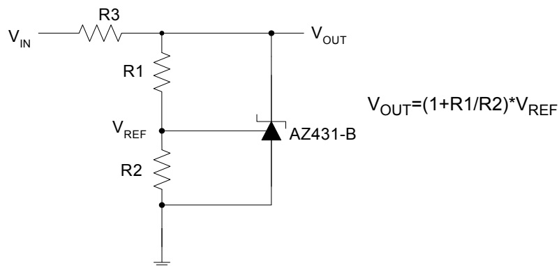
Figure 19. Shunt Regulator
