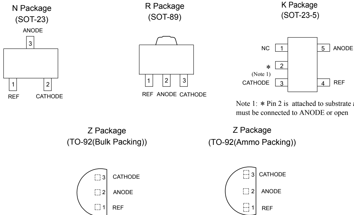
Figure 2. Pin Configuration of AZ431-B (Top View)
