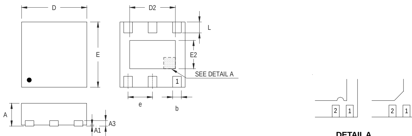
DETAIL A
