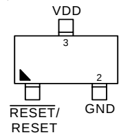
SOT-23-3 (L-Type)
