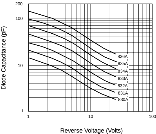
Diode Capacitance
