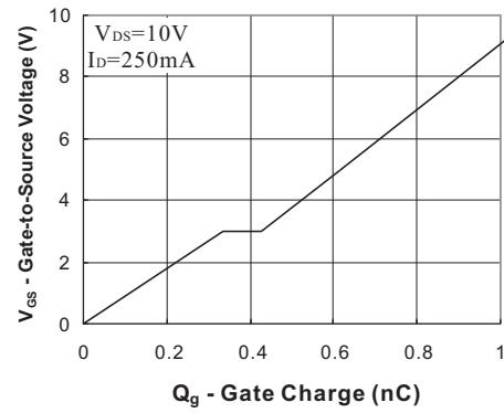
Fig.7 - Gate Charge
