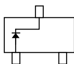
TOP VIEW BAT54
