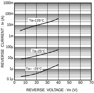
Fig.10 Reverse characteristics
