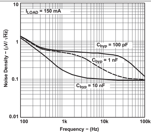
Figure 14. Output Noise Density vs Frequency
