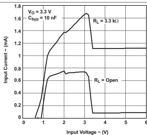
Figure 16. Input Current vs Input Voltage
