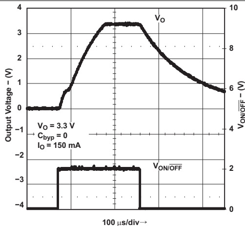
Figure 28. Turn-on Time
