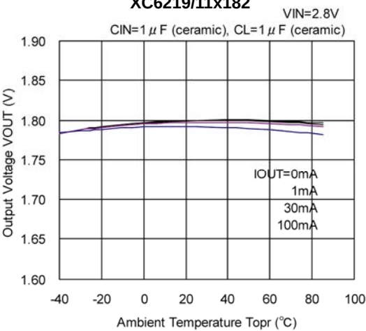
XC6219/11x182
