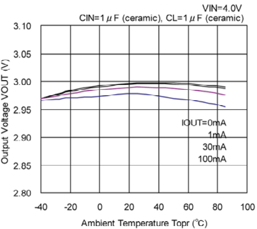
XC6219/11x302
