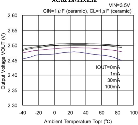
XC6219/11x252
