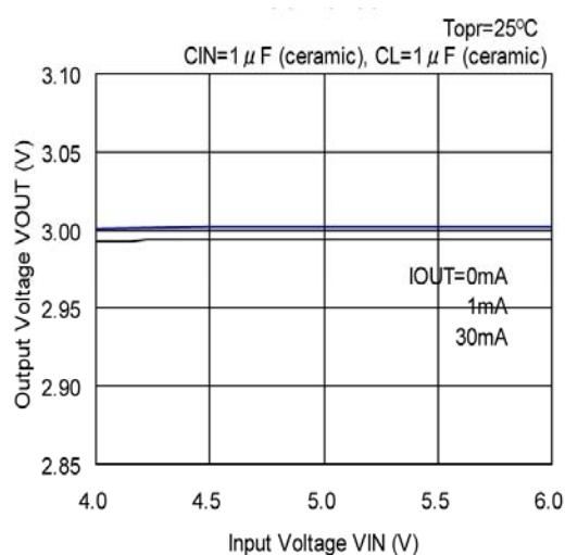
XC6219/11x302
