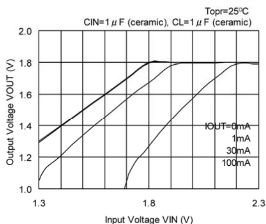
XC6219/11x182
