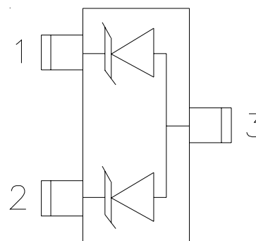
SOT23 (Top View)
