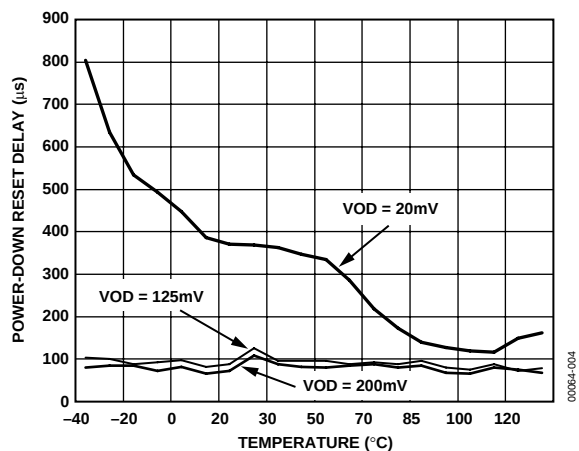
Figure 5. Power-Down Reset Delay vs. Temperature
