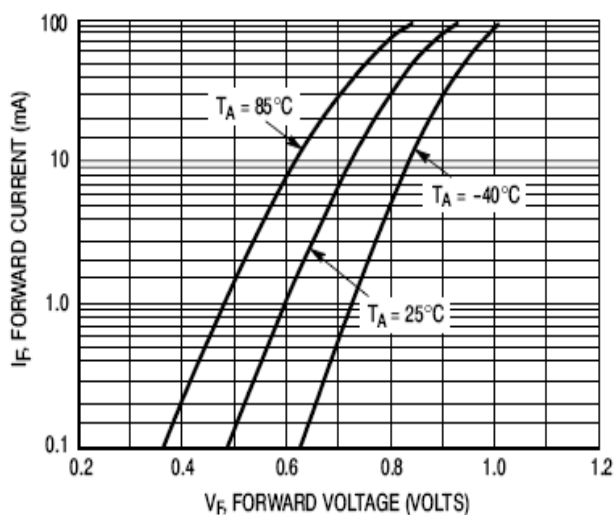
Figure 2. Forward Voltage
