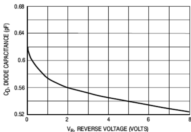
Figure 4. Diode Capacitance
