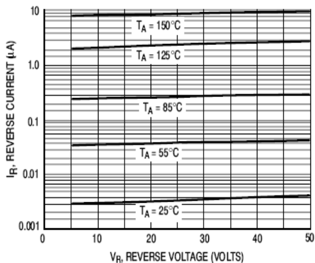
Figure 3. Reverse Current
