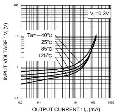
Fig.2 Input Voltage vs. Output Current
