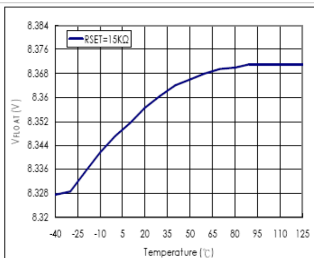
Regulated Output Voltage vs. Temperature
