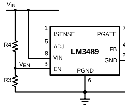
Figure 29. Adjustable UVLO
