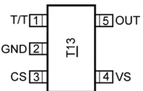
5-Pin TSOT-23 (D5) (Top View)
