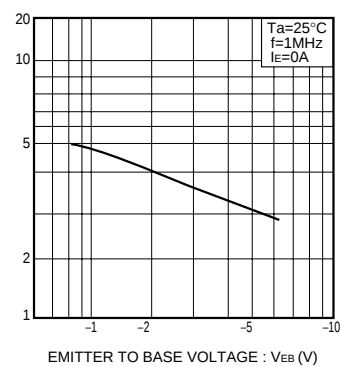
Fig.9 Emitter input capacitance vs. emitter-base voltage
