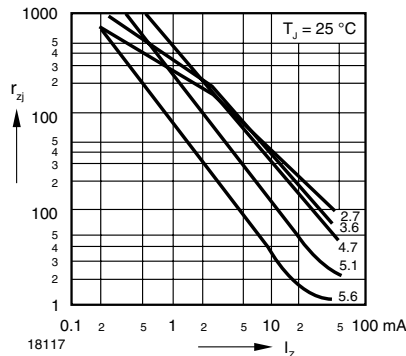
Figure 4. Dynamic Resistance vs. Zener Current
