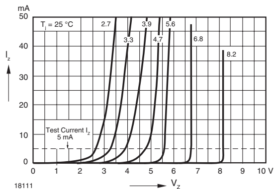
Figure 16. Breakdown Characteristics
