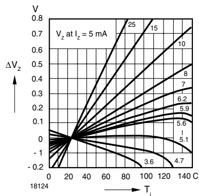
Figure 11. Change of Zener Voltage vs. Junction Temperature
