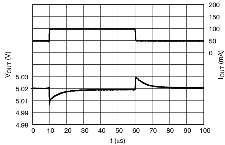
Figure 32. Load Transients, 5.0 V Version, I_{OUT} = 50 - 100 \text{ mA} , t_R = t_F = 0.5 \mu s , V_{IN} = 6.0 \text{ V}
