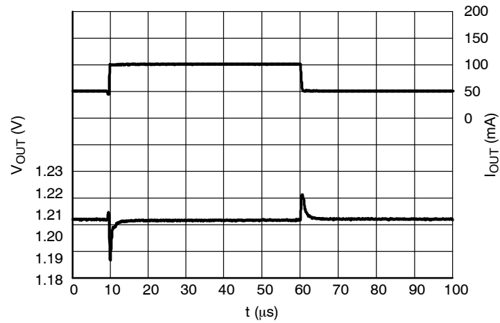
Figure 30. Load Transients, 1.2 V Version, I_{OUT} = 50 - 100 \text{ mA} , t_R = t_F = 0.5 \mu s , V_{IN} = 2.2 \text{ V}
