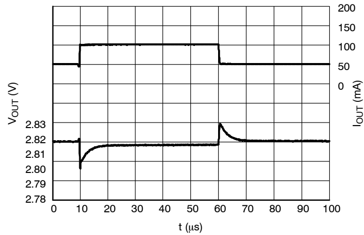
Figure 31. Load Transients, 2.8 V Version, I_{OUT} = 50 - 100 \text{ mA} , t_R = t_F = 0.5 \mu s , V_{IN} = 3.8 \text{ V}
