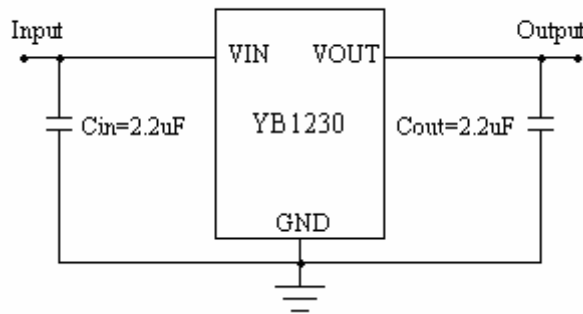
Figure 1-2: SOT-23/SOT-89 Application Circuit
