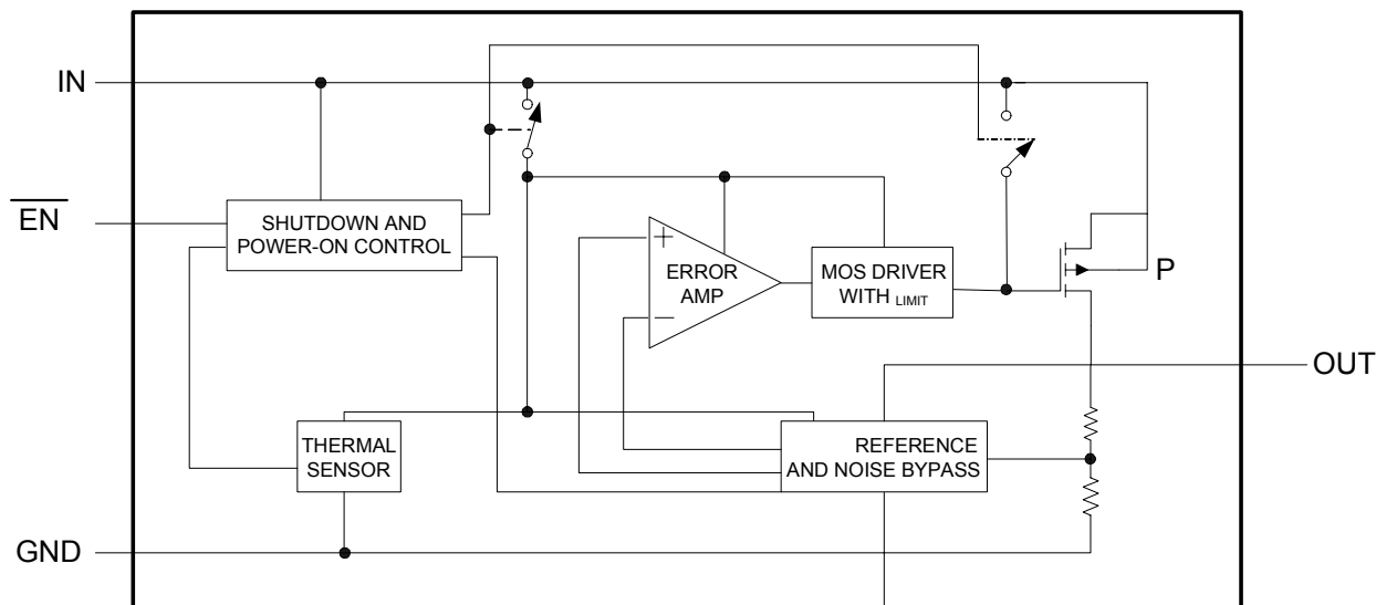
Figure 3: Function Block
