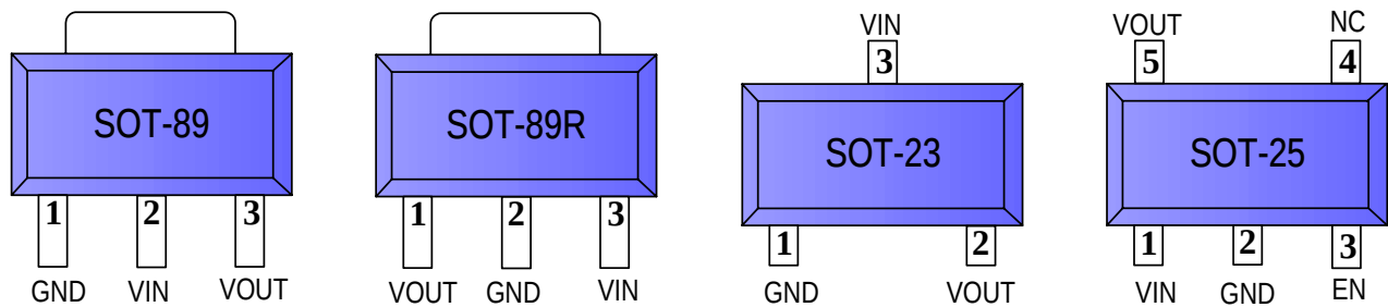
Figure 2 : pin configuration
